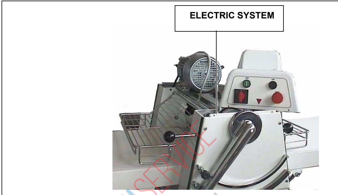
Fig. 4.2 Electric system position
